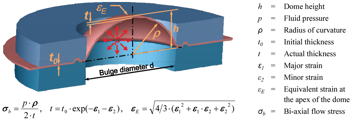
Figure 2: Extended bulge test used for yield curve determination.
