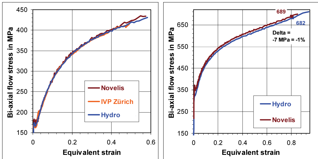
Figure 12: Comparison of biaxial flow curves measured in different laboratories
